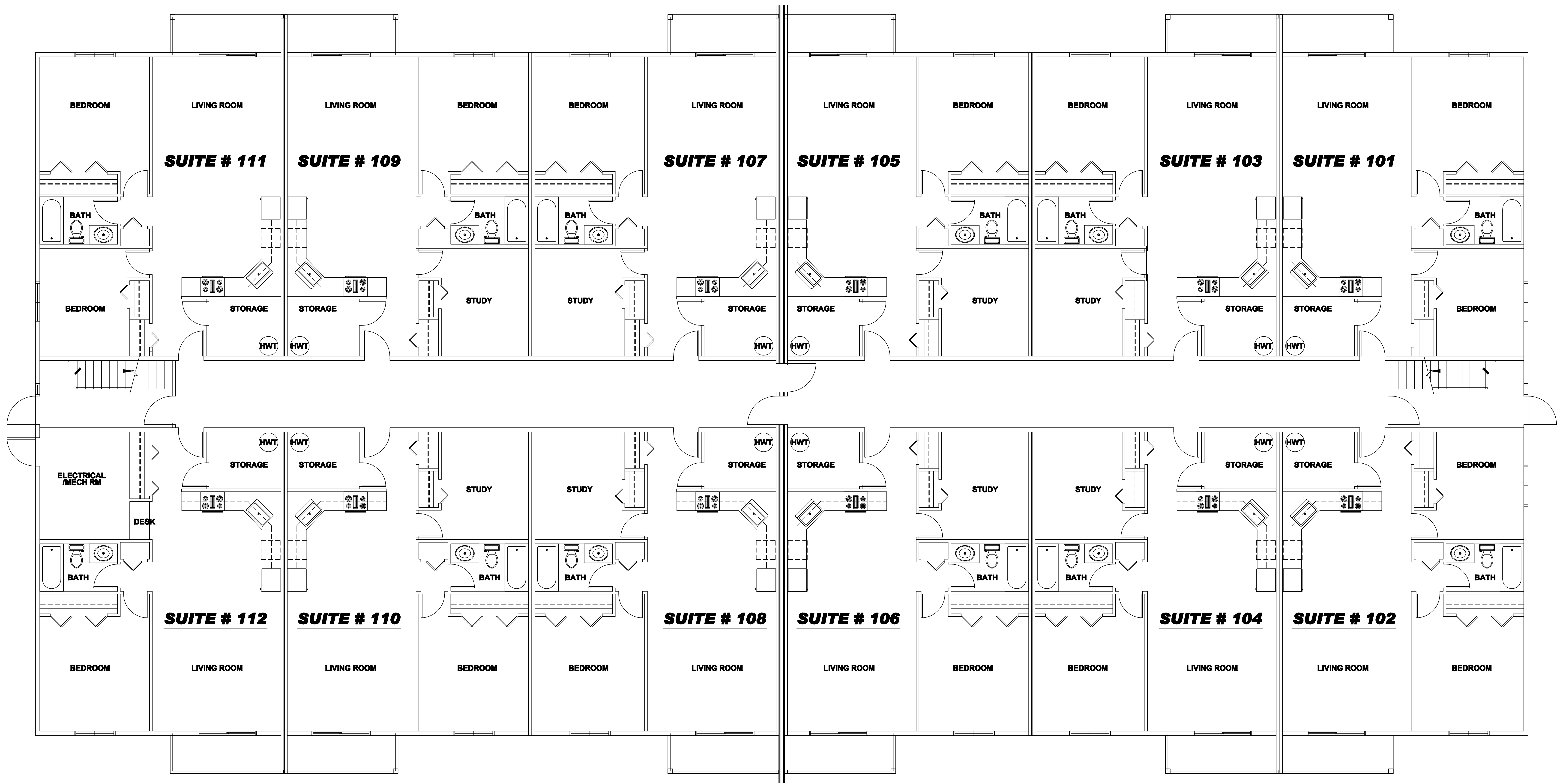
MAIN FLOOR PLAN SCALE: 1/8" = 1'-0"
